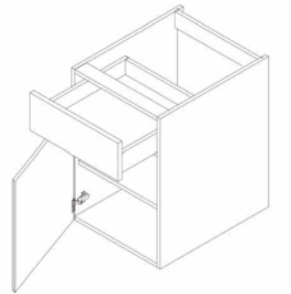
Single-door Base Cabinet With One Drawer
