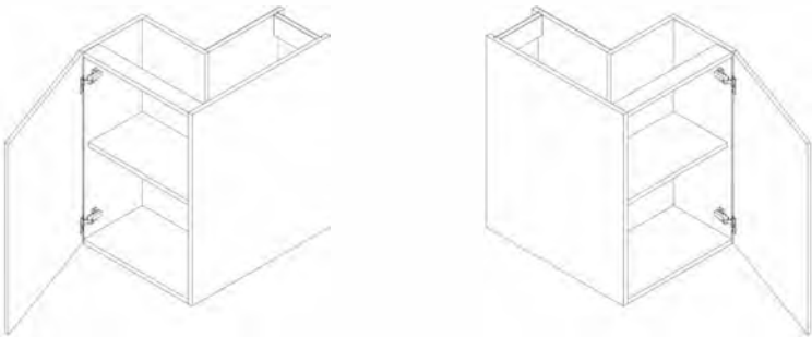
Single-door Unfilled Corner Blind Base Cabinet
