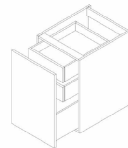
Single-drawer Base Cabinet With Two Small Built-in Drawers
