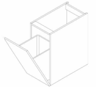
Base Cabinet For Oblique Opening Waste Bin
