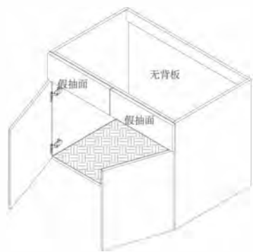
Sink Base Cabinet With 2 Doors And 2 Dummy Drawers
